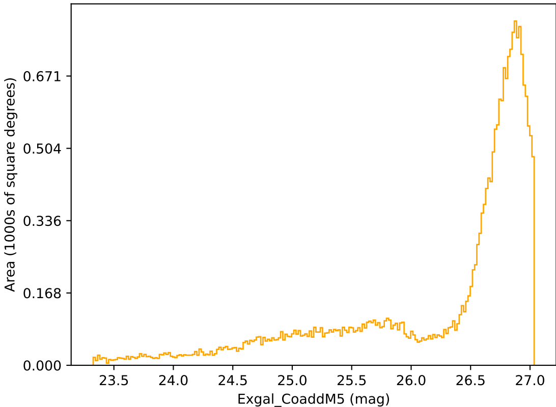
too_elab_r256_d3_giz_v3.4_10yrs All sky r band: Exgal_CoaddM5
