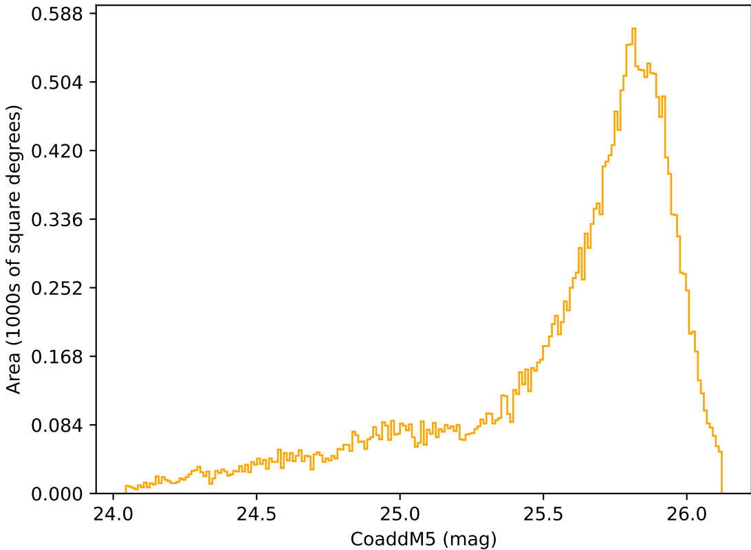
too_elab_r256_d3_giz_v3.4_10yrs Yr 1 r band: CoaddM5
