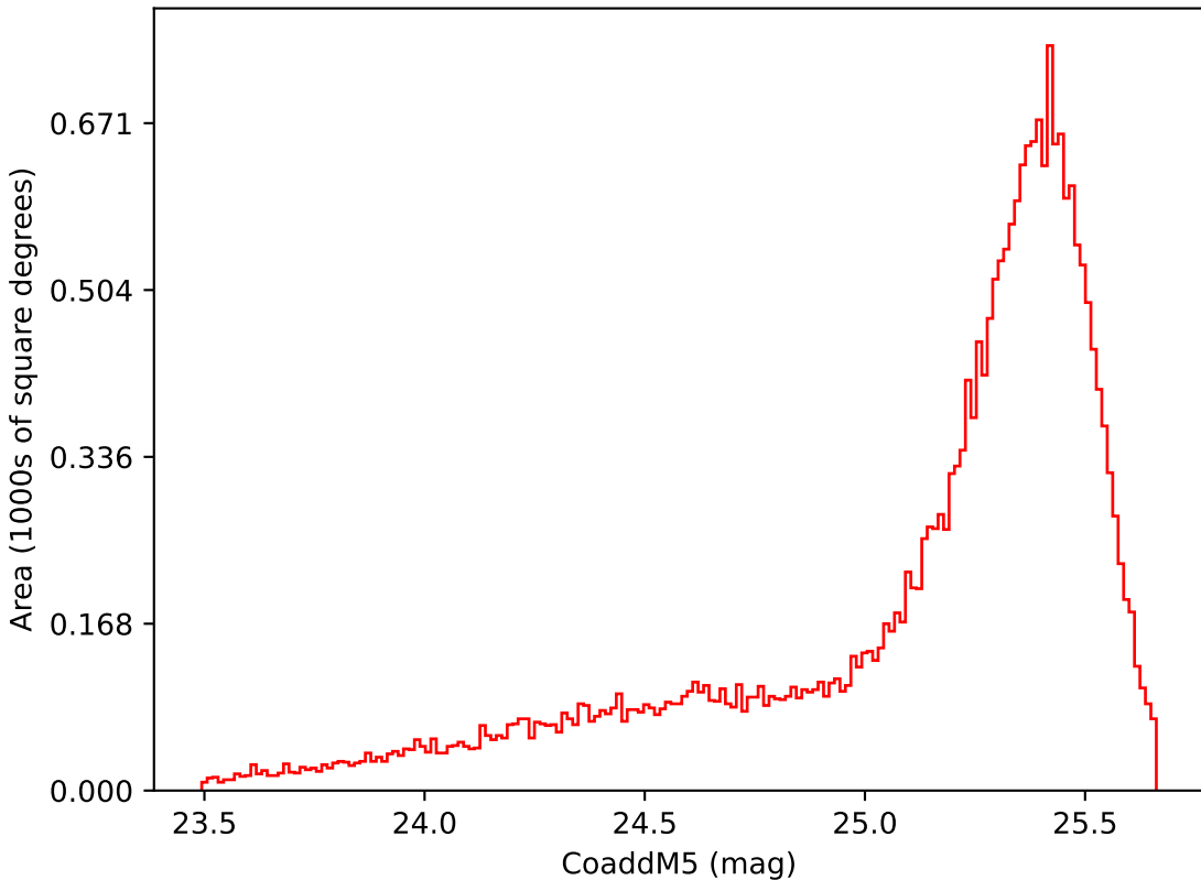
too_elab_r256_d3_giz_v3.4_10yrs Yr 1 i band: CoaddM5
