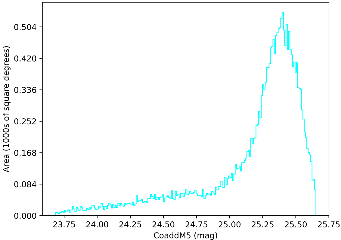
too_elab_r256_d3_giz_v3.4_10yrs All sky u band: CoaddM5
