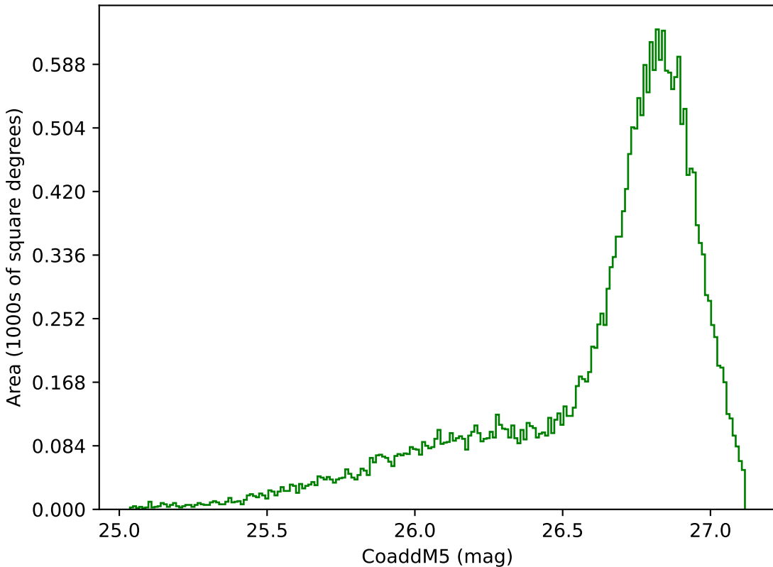
too_elab_r256_d3_giz_v3.4_10yrs All sky g band: CoaddM5
