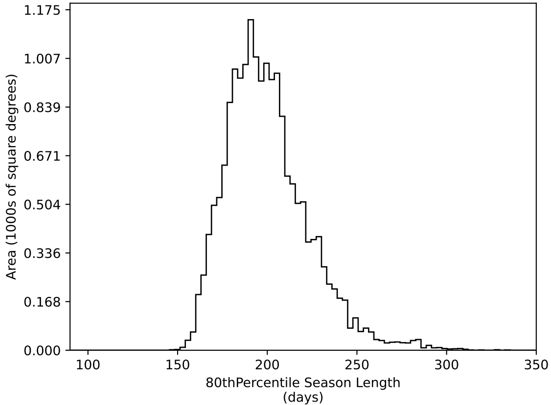
too_elab_r256_d3_giz_v3.4_10yrs WFD all bands: 80thPercentile Season Length
