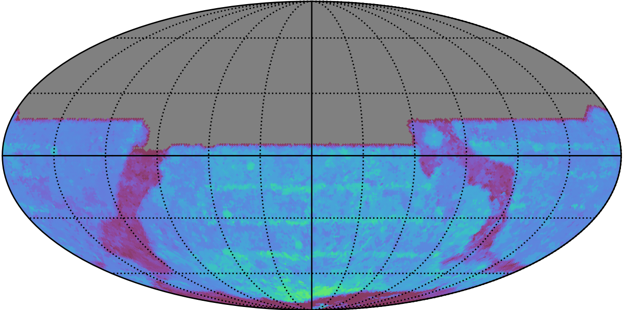
too_elab_r256_d3_giz_v3.4_10yrs All sky y band: 80thPercentile Season Length
