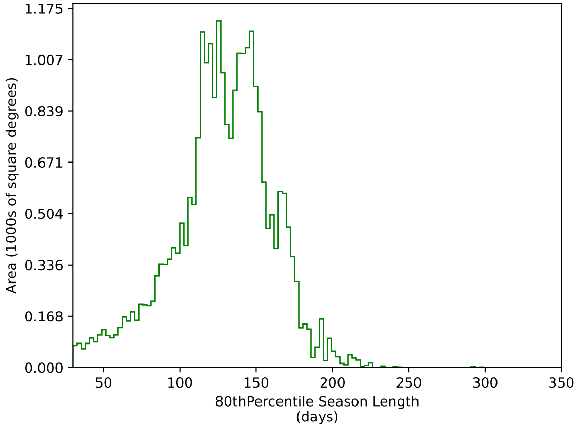
too_elab_r256_d3_giz_v3.4_10yrs All sky g band: 80thPercentile Season Length
