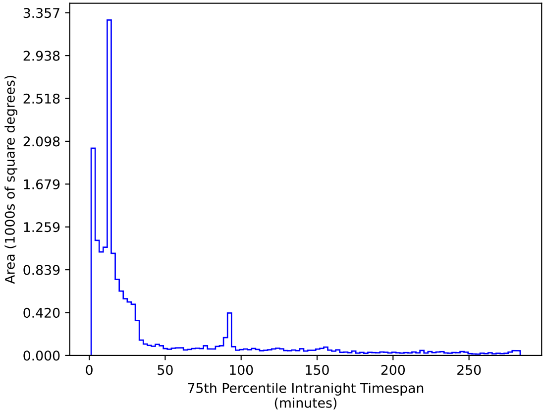
too_elab_r256_d3_giz_v3.4_10yrs WFD r band: 75th Percentile Intranight Timespan
