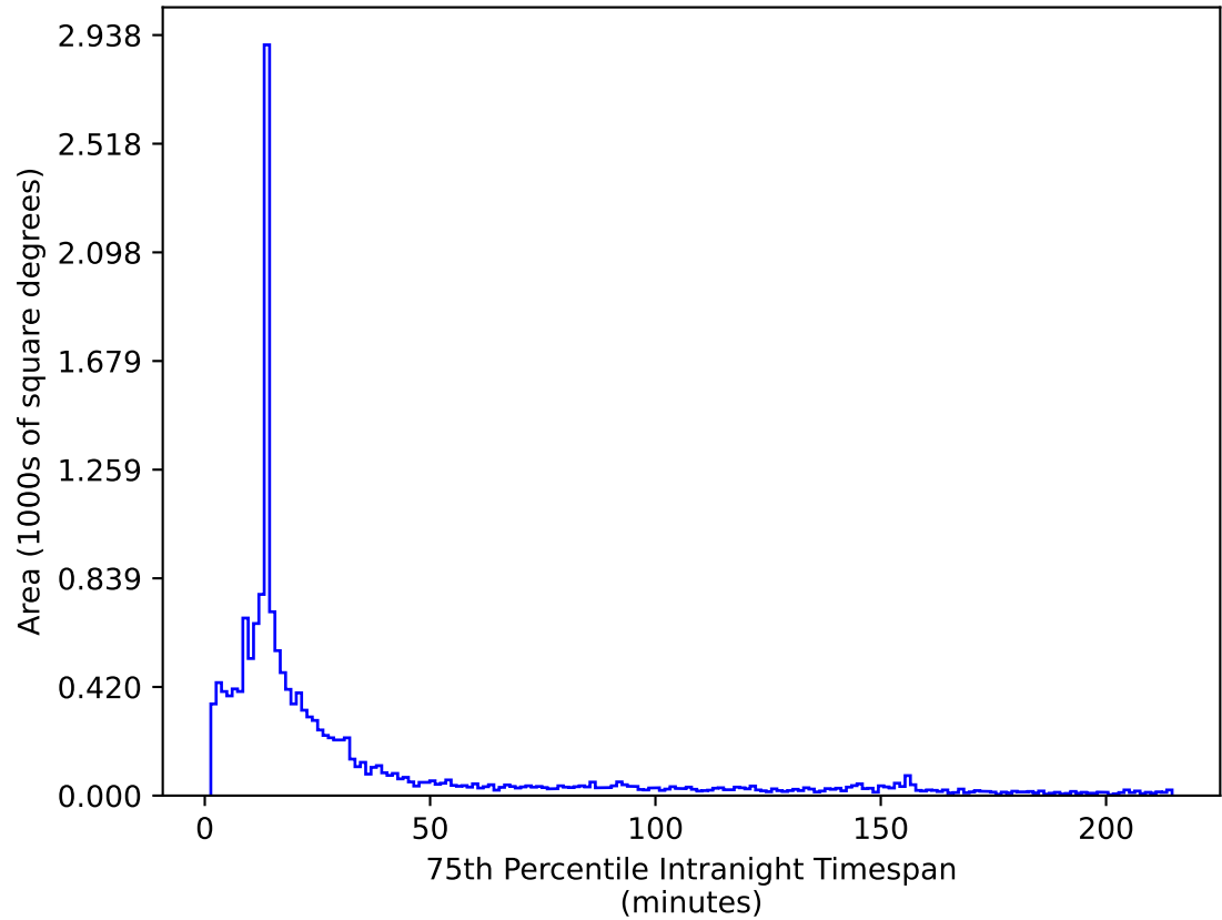
too_elab_r256_d3_giz_v3.4_10yrs WFD i band: 75th Percentile Intranight Timespan
