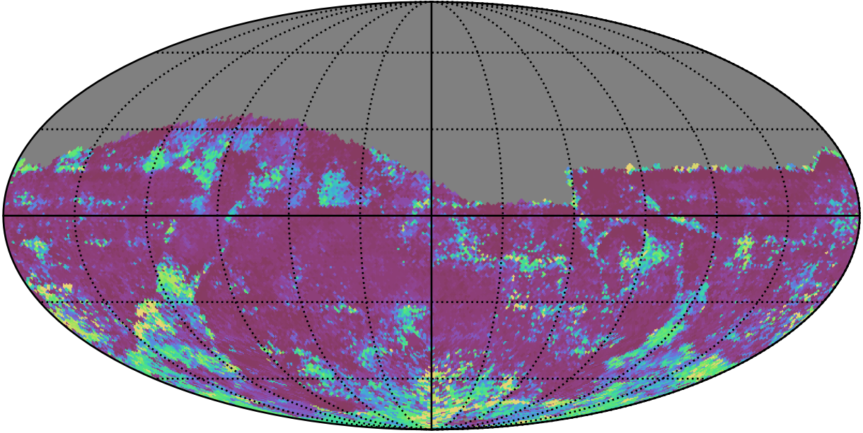
too_elab_r256_d3_giz_v3.4_10yrs All sky z band: 75th Percentile Intranight Timespan
