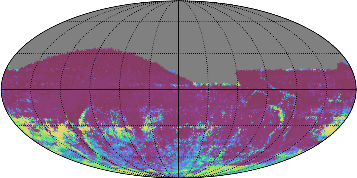
too_elab_r256_d3_giz_v3.4_10yrs All sky r band: 75th Percentile Intranight Timespan
