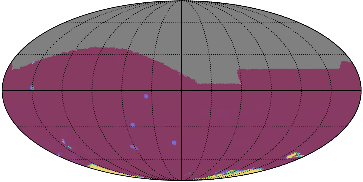
too_elab_r256_d3_giz_v3.4_10yrs All sky all bands: 75th Percentile Intranight Timespan
