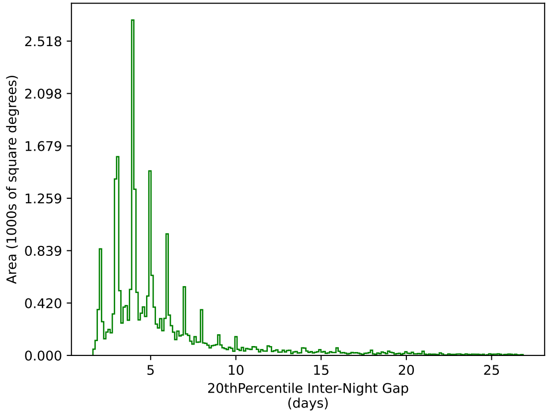
too_elab_r256_d3_giz_v3.4_10yrs All sky g band: 20thPercentile Inter-Night Gap
