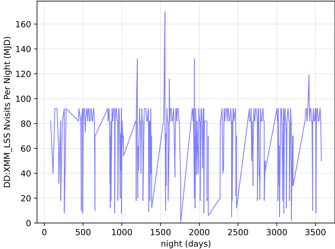
too_elab_r256_d3_giz_v3.4_10yrs all bands: DD:XMM_LSS Nvisits Per Night
