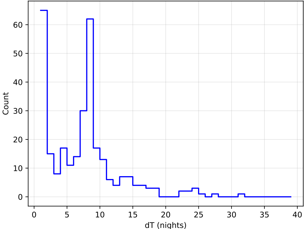
too_elab_r256_d3_giz_v3.4_10yrs all bands: DD:XMM_LSS Delta Nights Histogram
