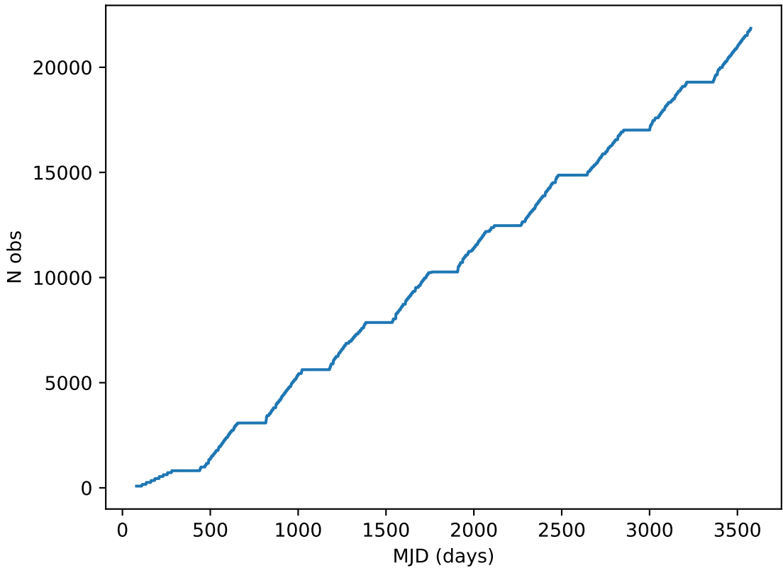
too_elab_r256_d3_giz_v3.4_10yrs all bands: DD:XMM_LSS Cumulative NVisits
