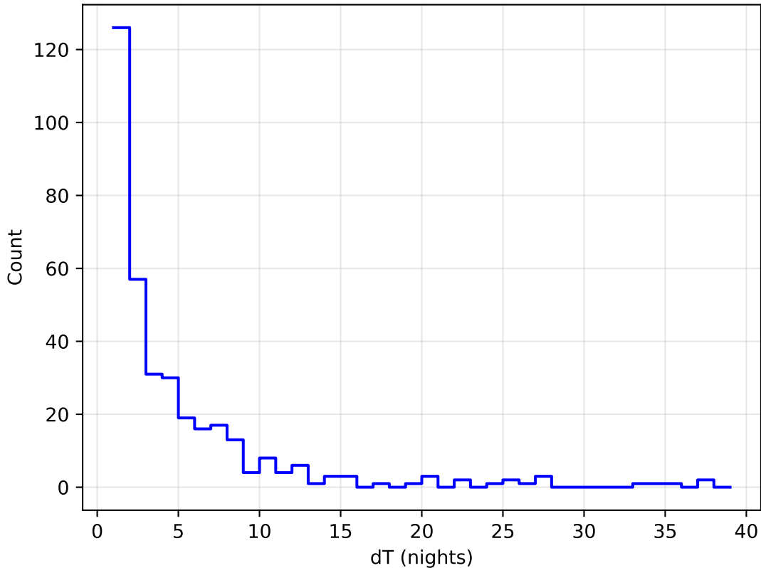
too_elab_r256_d3_giz_v3.4_10yrs all bands: DD:WFD Delta Nights Histogram
