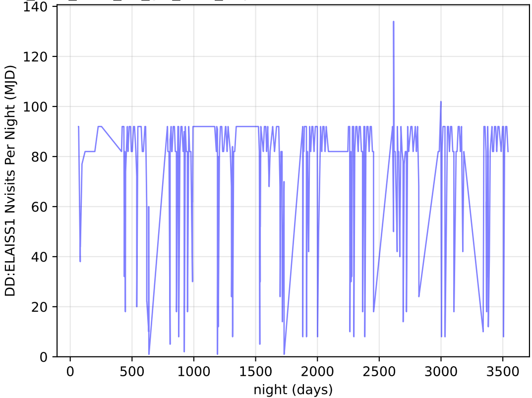
too_elab_r256_d3_giz_v3.4_10yrs all bands: DD:ELAISS1 Nvisits Per Night
