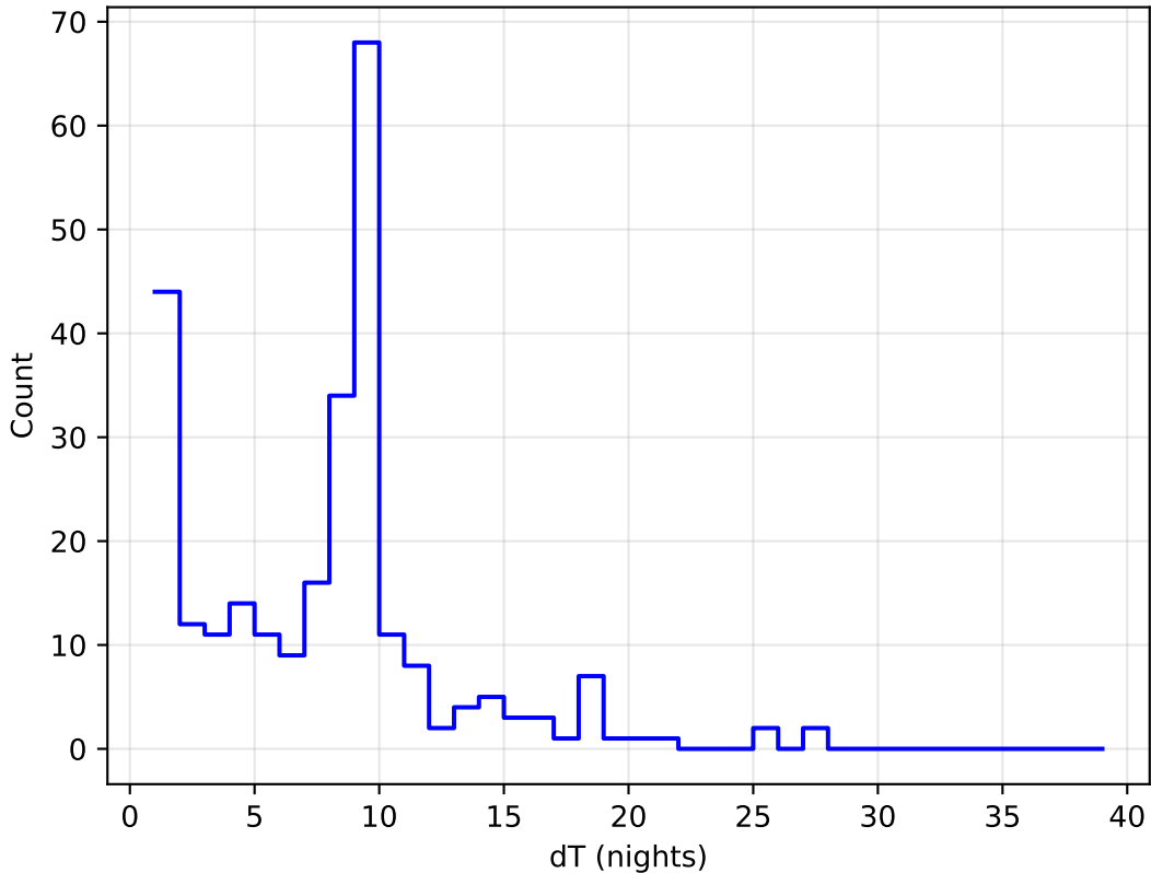
too_elab_r256_d3_giz_v3.4_10yrs all bands: DD:ELAISS1 Delta Nights Histogram
