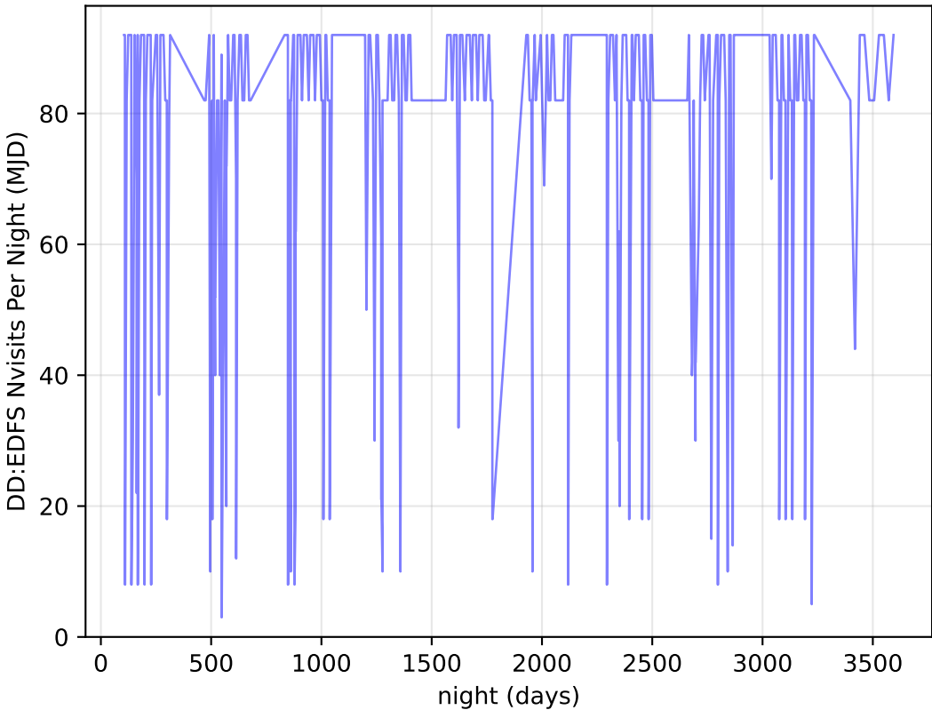
too_elab_r256_d3_giz_v3.4_10yrs all bands: DD:EDFS Nvisits Per Night
