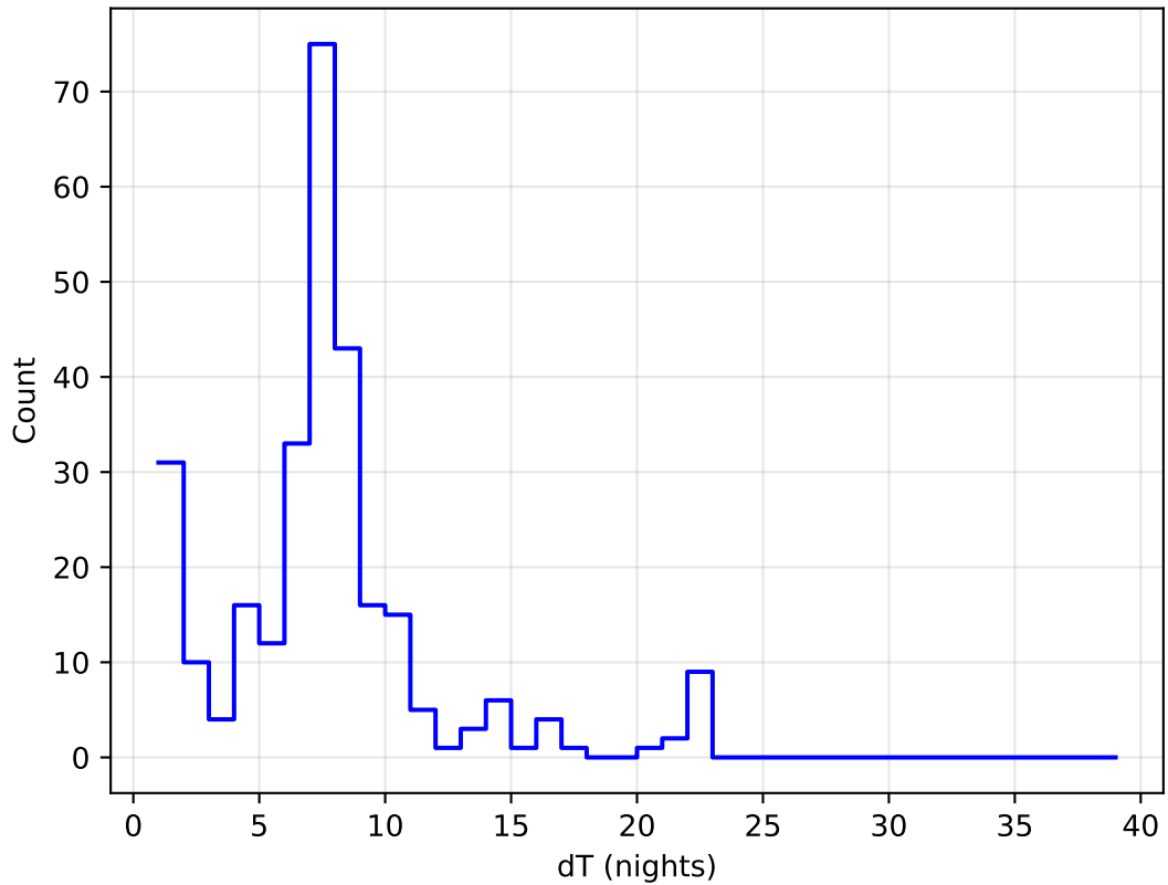
too_elab_r256_d3_giz_v3.4_10yrs all bands: DD:EDFS Delta Nights Histogram
