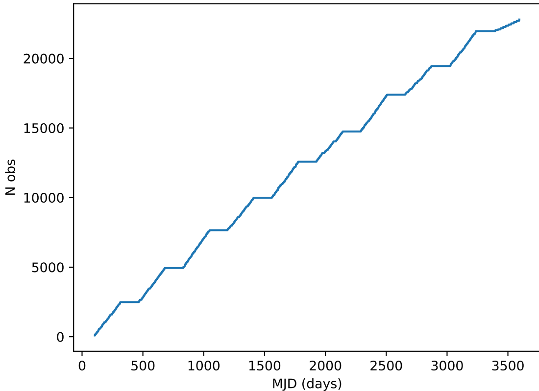
too_elab_r256_d3_giz_v3.4_10yrs all bands: DD:EDFS Cumulative NVisits
