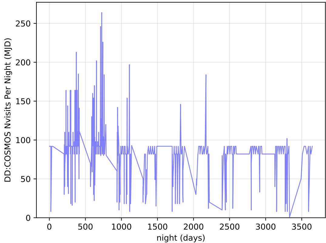
too_elab_r256_d3_giz_v3.4_10yrs all bands: DD:COSMOS Nvisits Per Night
