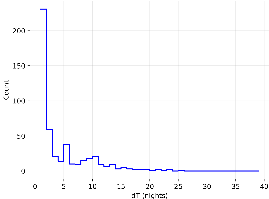
too_elab_r256_d3_giz_v3.4_10yrs all bands: DD: COSMOS Delta Nights Histogram
