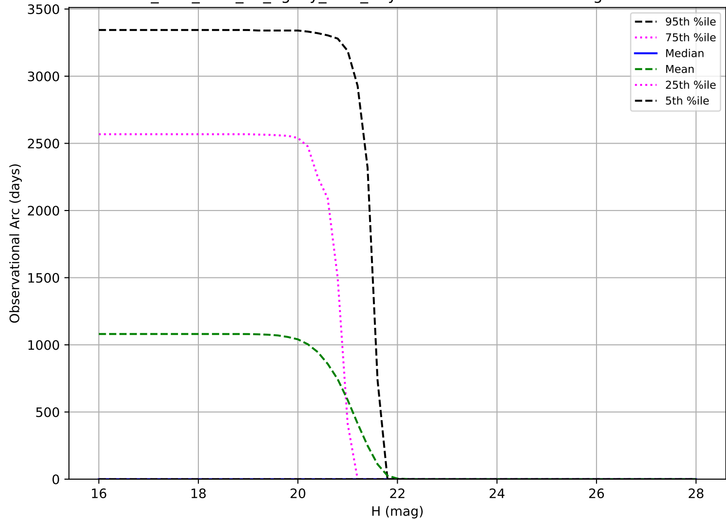
too_elab_r256_d2_ugrizy_v3.4_10yrs: Observational Arc Length Vatira
