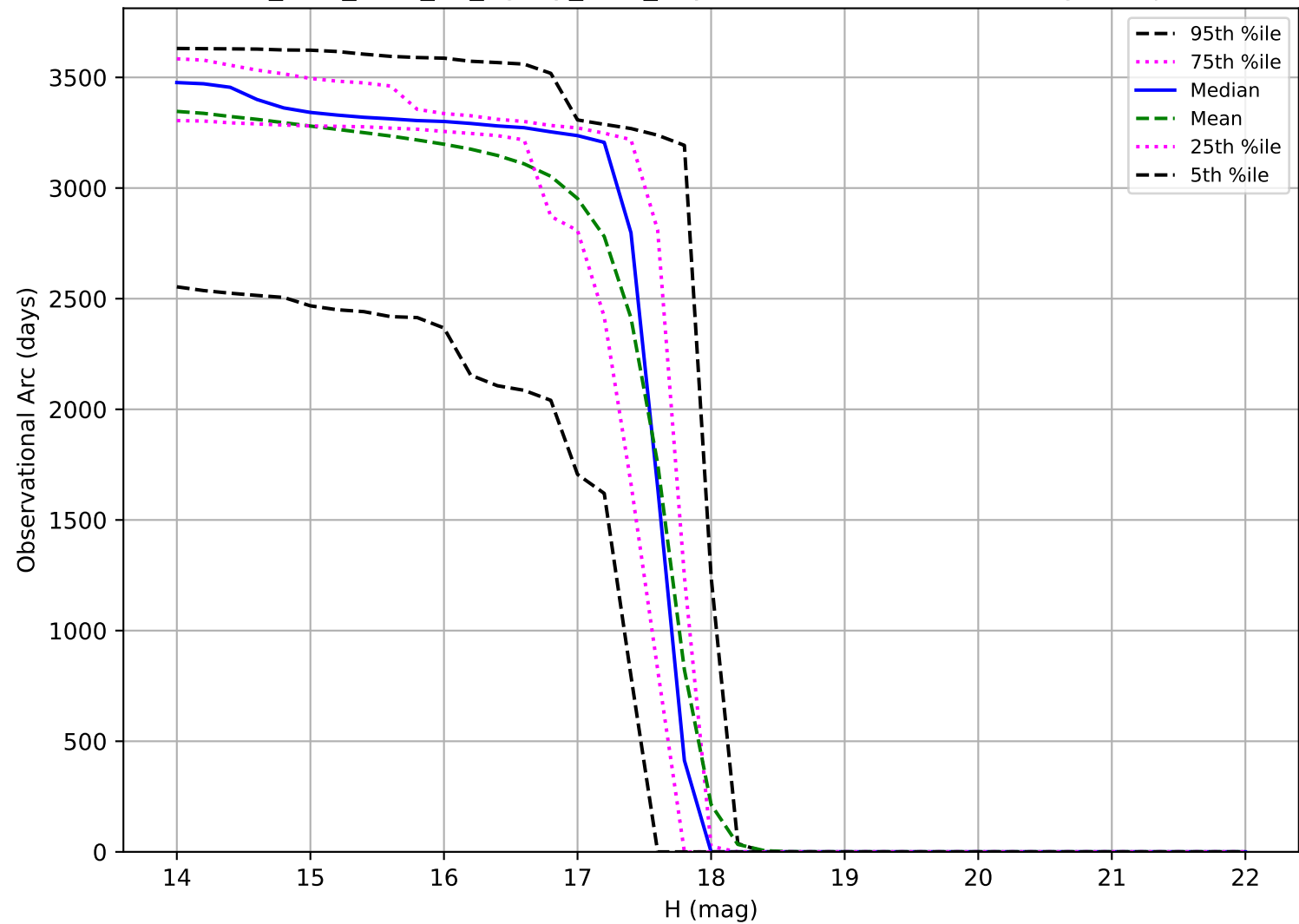
too_elab_r256_d2_ugrizy_v3.4_10yrs: Observational Arc Length Trojan
