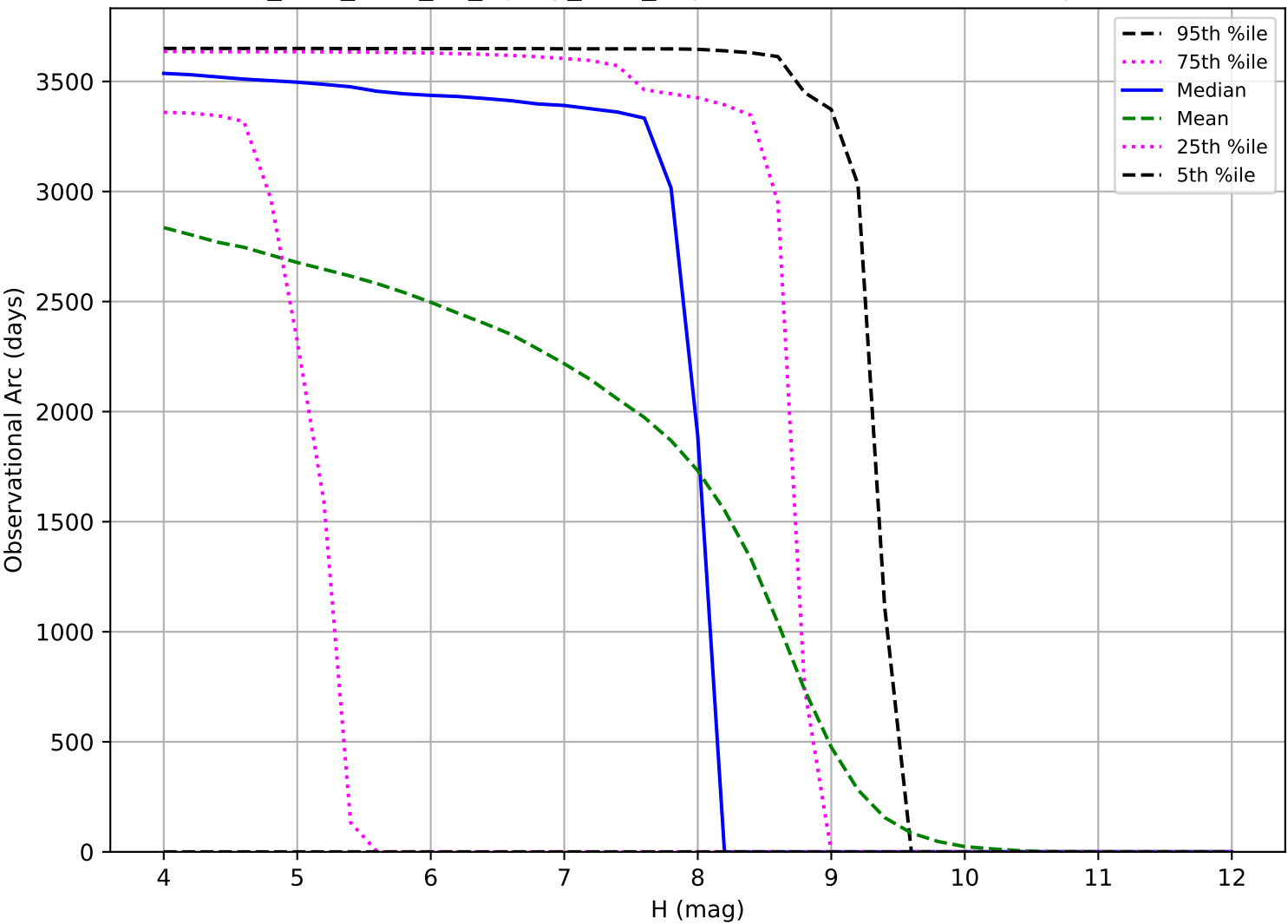
too_elab_r256_d2_ugrizy_v3.4_10yrs: Observational Arc Length TNO
