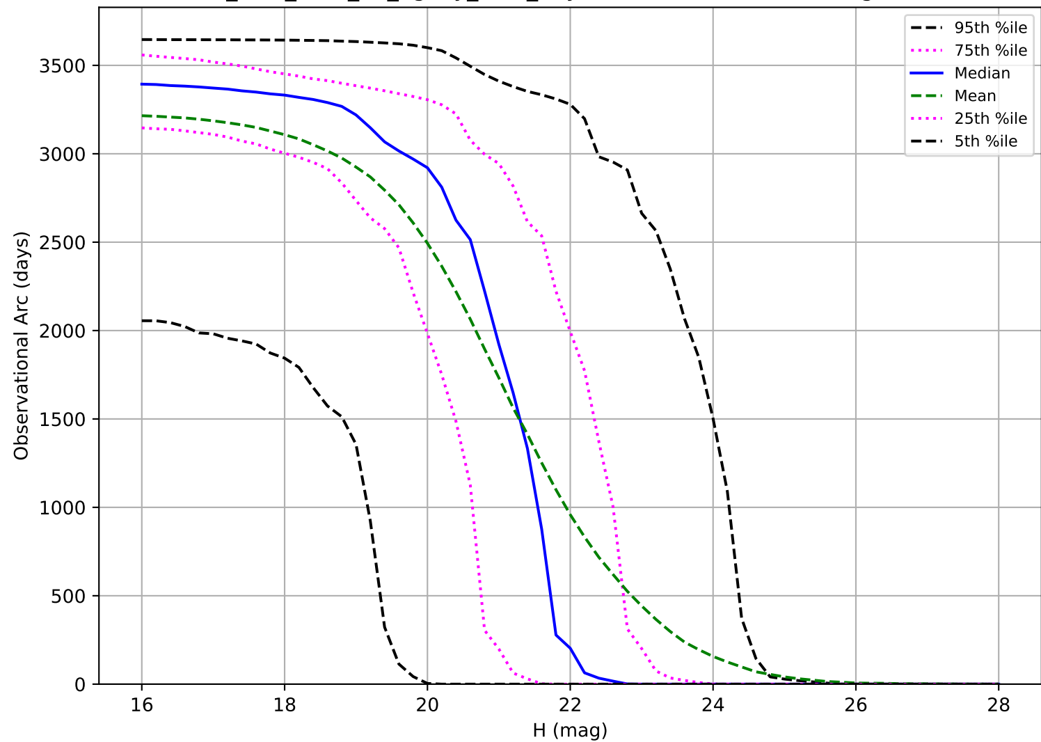
too_elab_r256_d2_ugrizy_v3.4_10yrs: Observational Arc Length PHA
