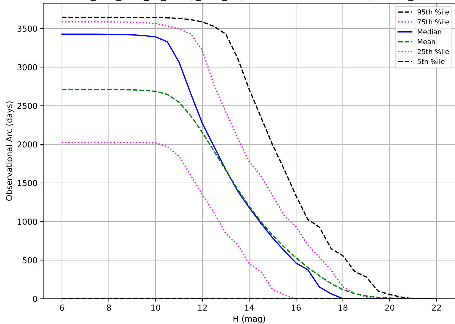
too_elab_r256_d2_ugrizy_v3.4_10yrs: Observational Arc Length OCC_r5
