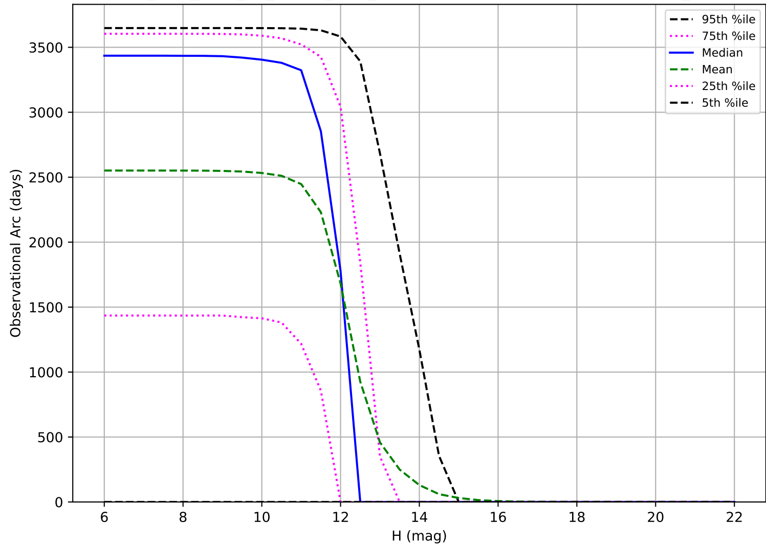
too_elab_r256_d2_ugrizy_v3.4_10yrs: Observational Arc Length OCC_r20
