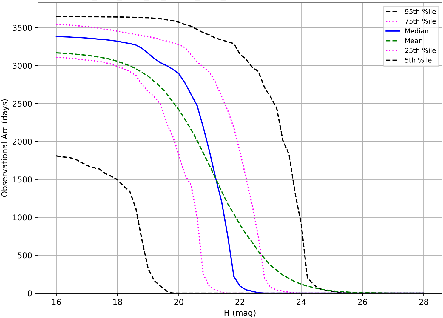
too_elab_r256_d2_ugrizy_v3.4_10yrs: Observational Arc Length NEO
