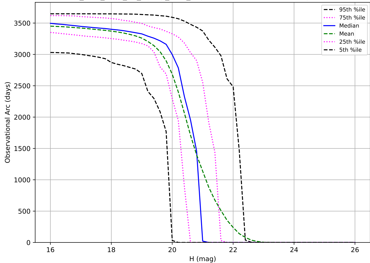
too_elab_r256_d2_ugrizy_v3.4_10yrs: Observational Arc Length MBA
