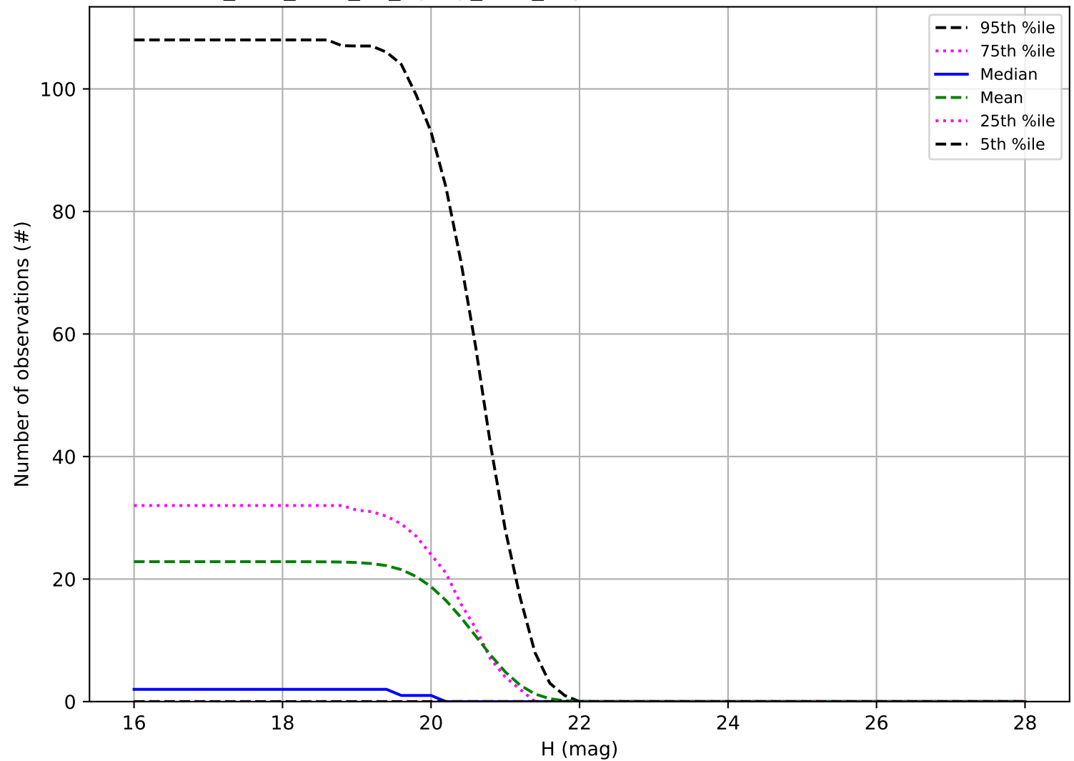
too_elab_r256_d2_ugrizy_v3.4_10yrs: Number of observations Vatira
