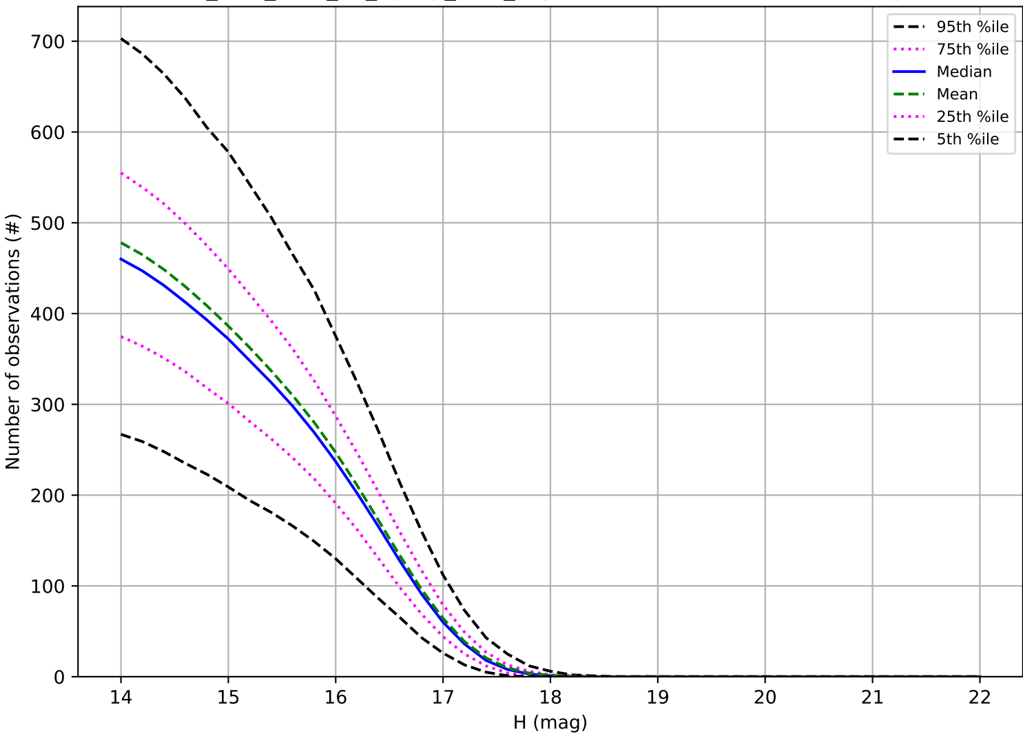
too_elab_r256_d2_ugrizy_v3.4_10yrs: Number of observations Trojan
