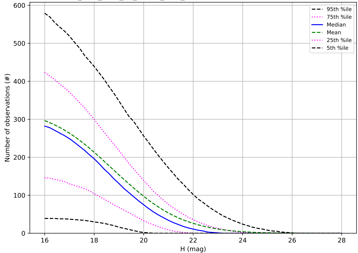
too_elab_r256_d2_ugrizy_v3.4_10yrs: Number of observations PHA
