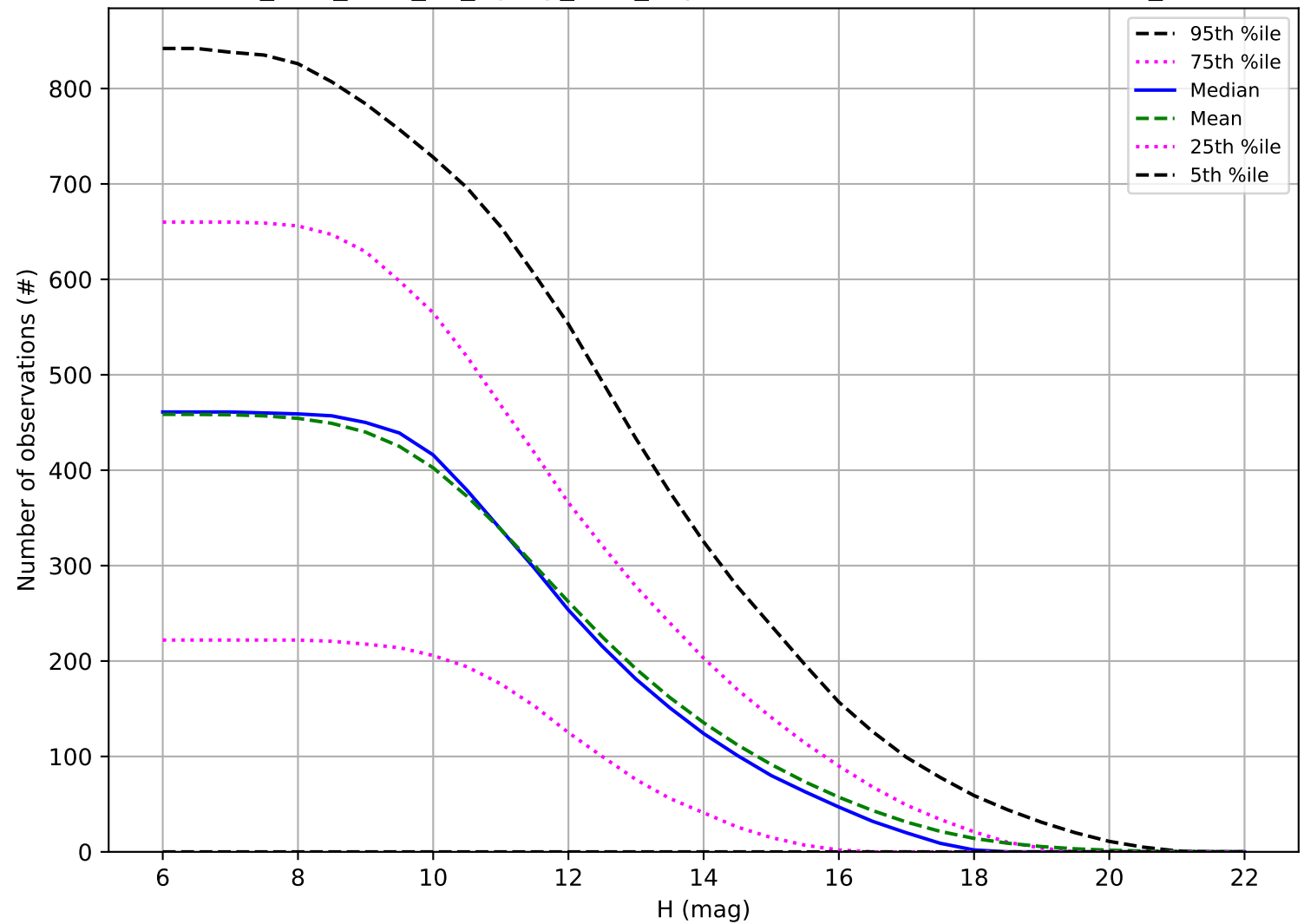
too_elab_r256_d2_ugrizy_v3.4_10yrs: Number of observations OCC_r5
