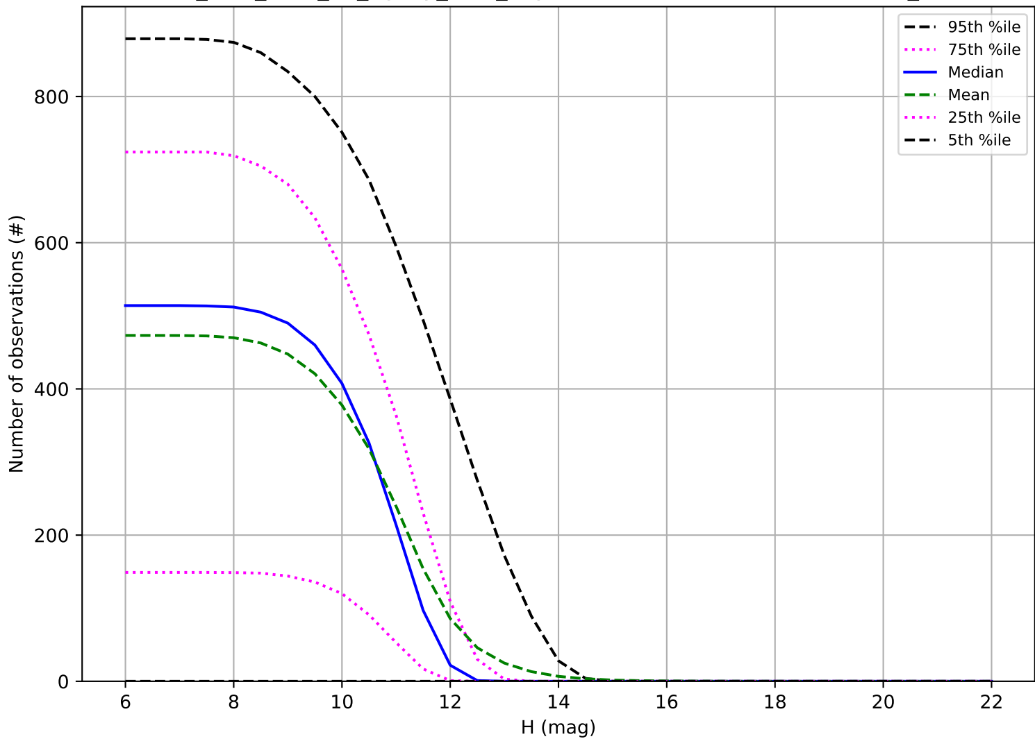
too_elab_r256_d2_ugrizy_v3.4_10yrs: Number of observations OCC_r20
