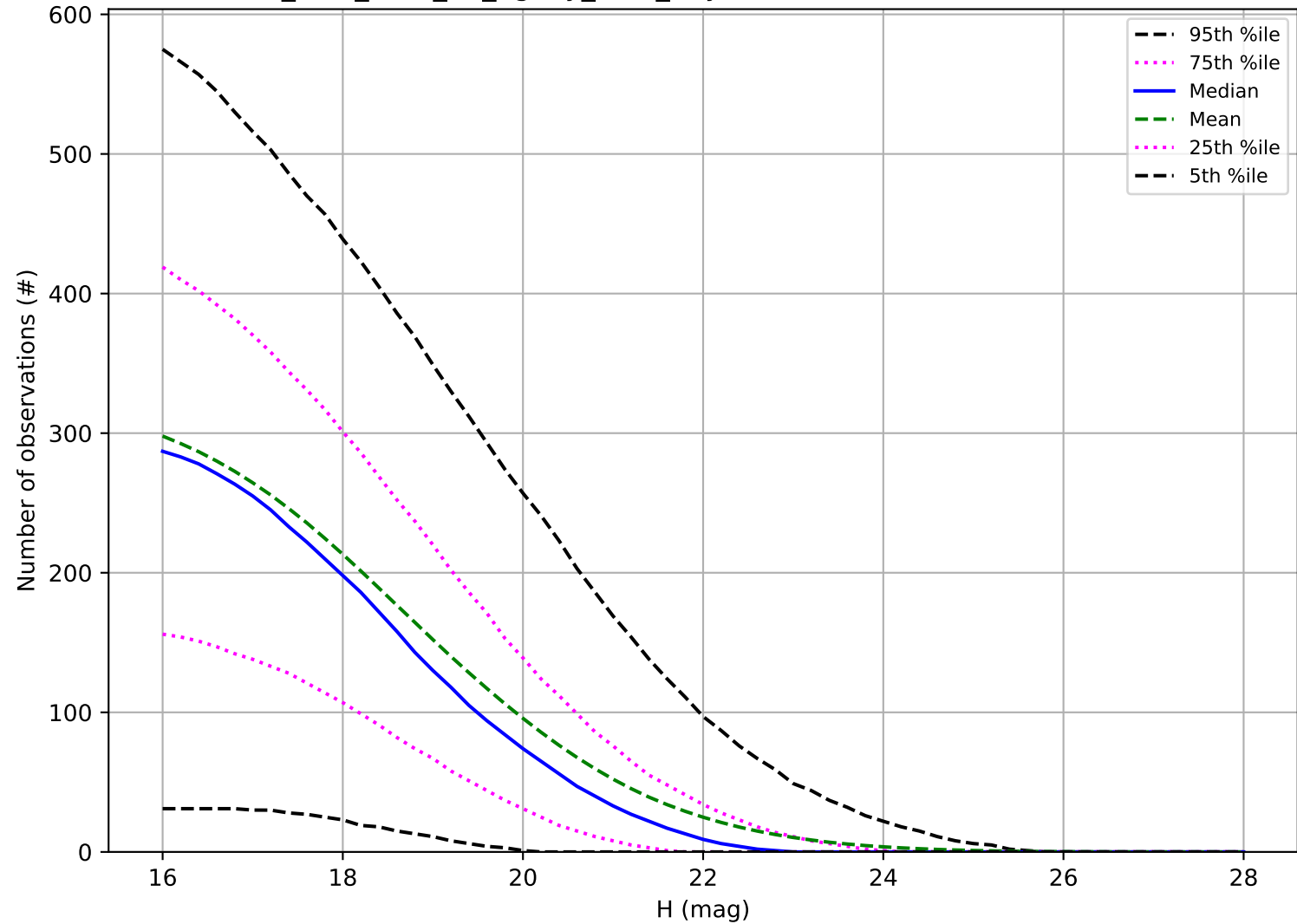
too_elab_r256_d2_ugrizy_v3.4_10yrs: Number of observations NEO
