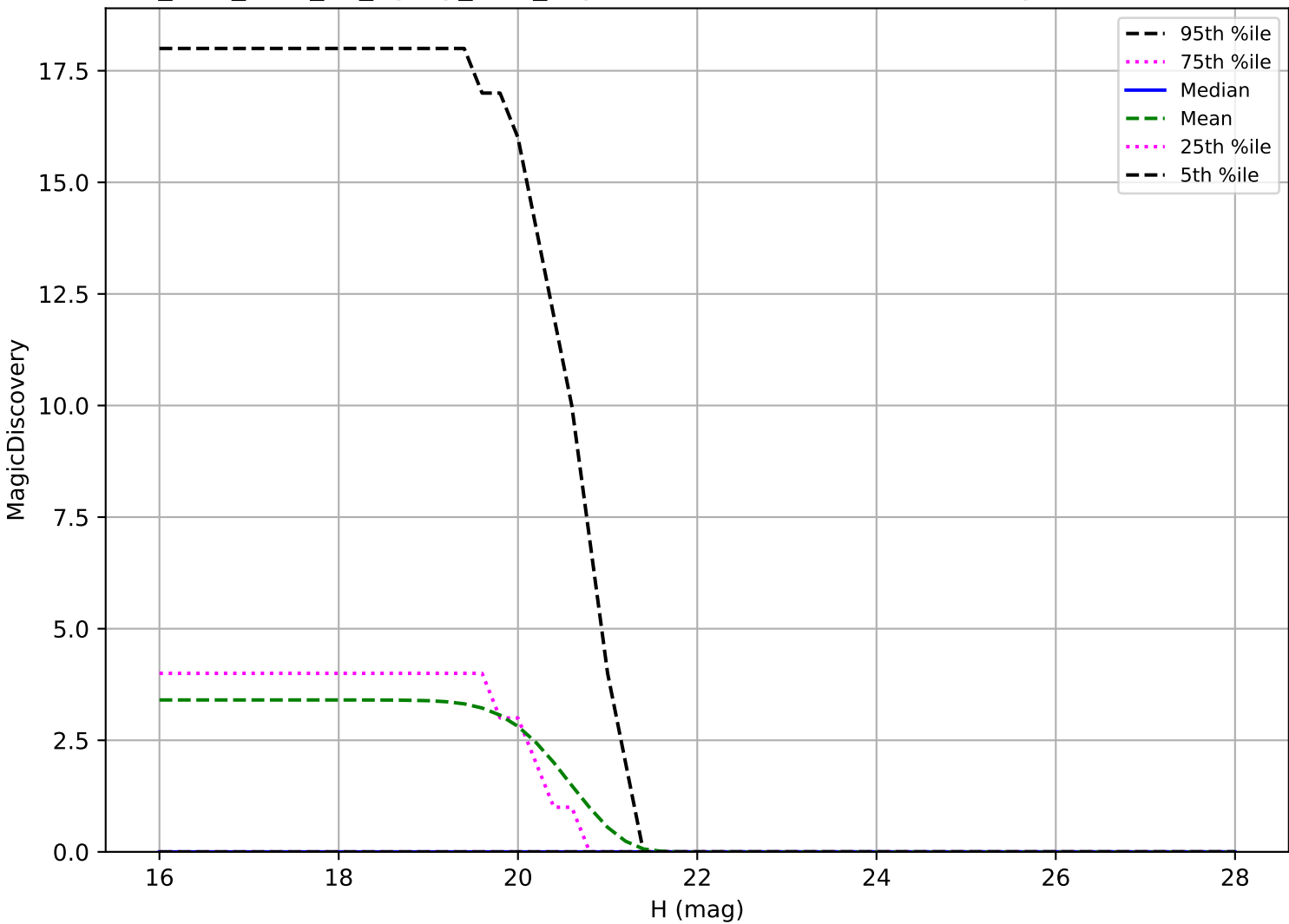
too_elab_r256_d2_ugrizy_v3.4_10yrs: Vatira 6 detections in 60 nights detection loss
