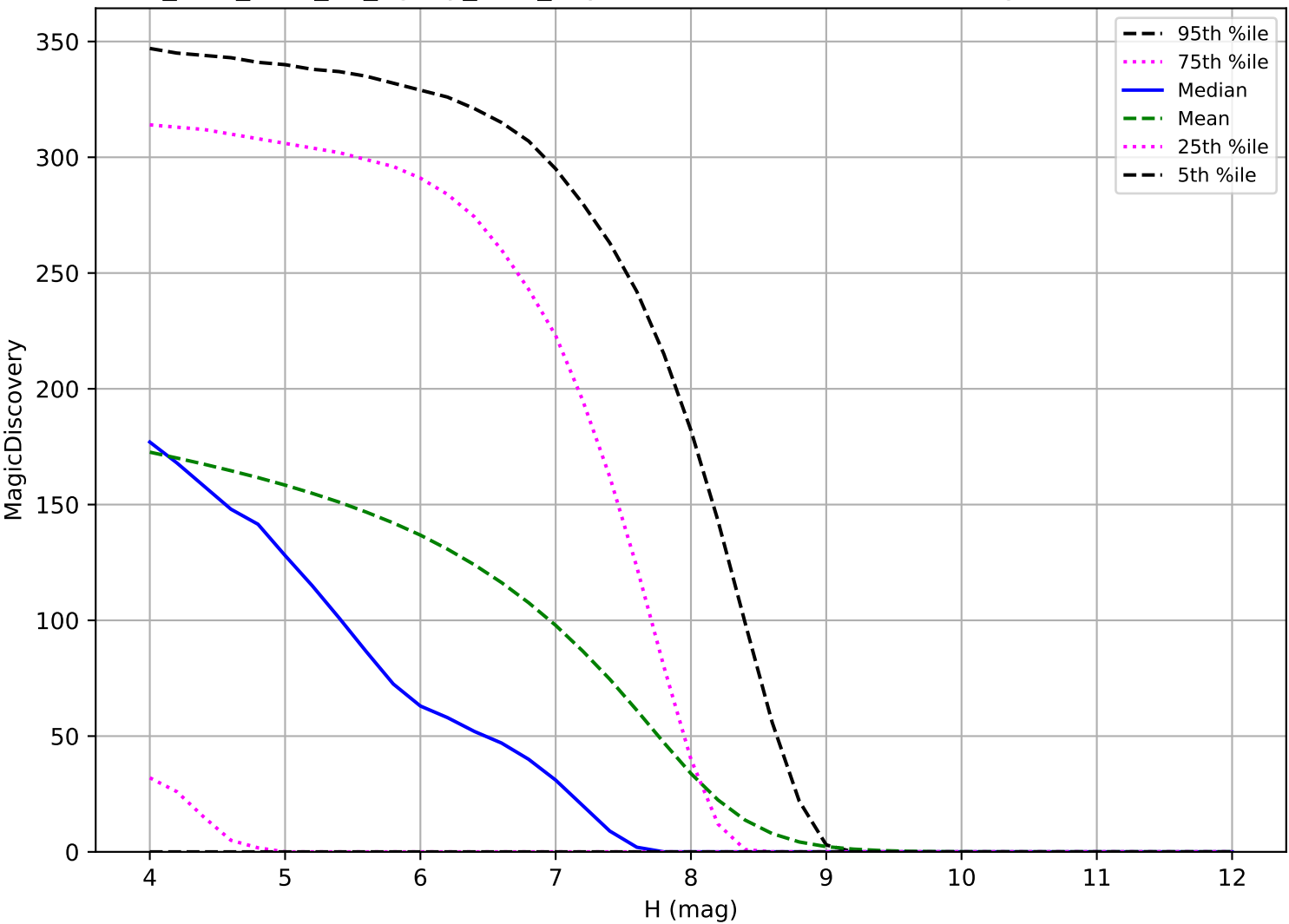
too_elab_r256_d2_ugrizy_v3.4_10yrs: TNO 6 detections in 60 nights detection loss
