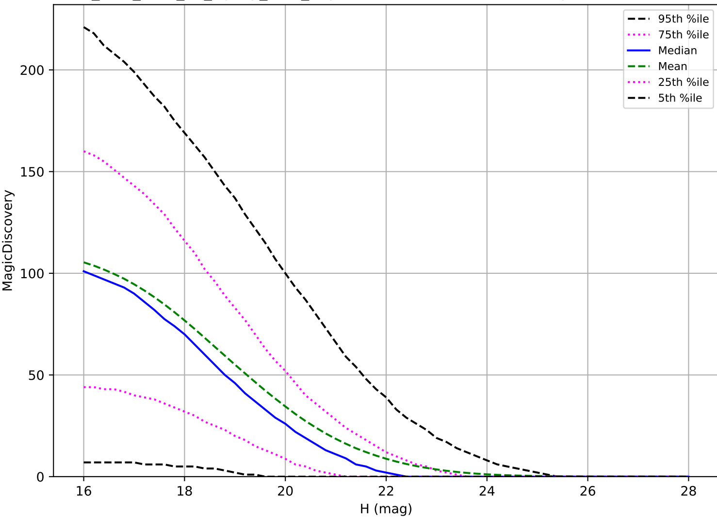
too_elab_r256_d2_ugrizy_v3.4_10yrs: PHA 6 detections in 60 nights detection loss
