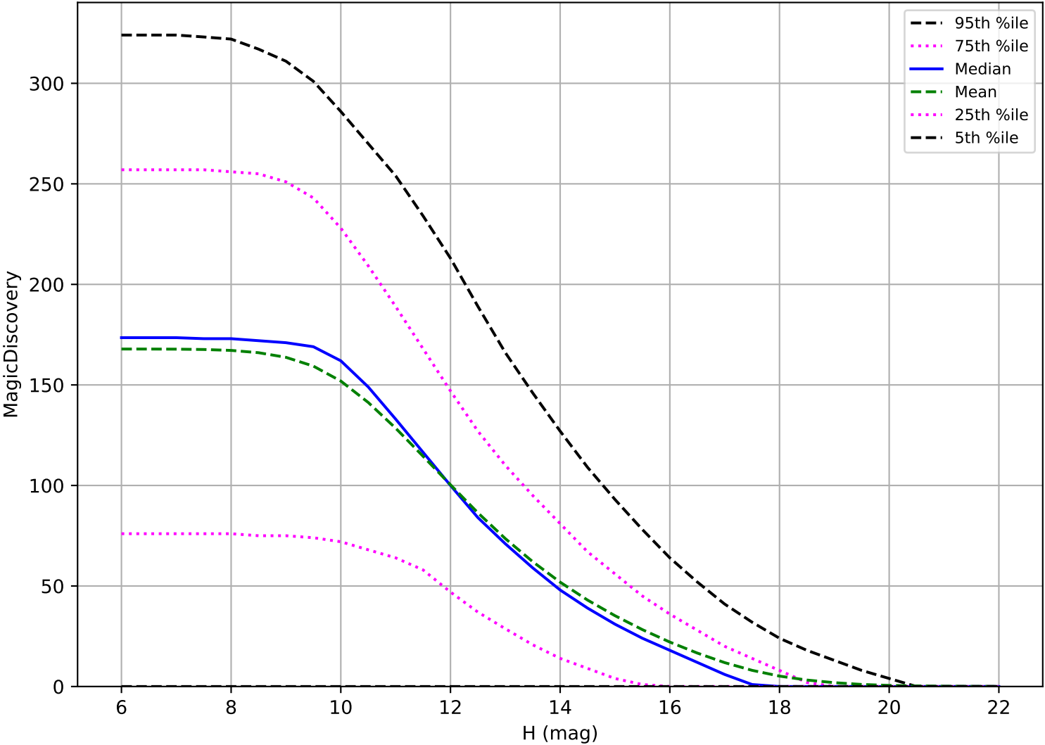
too_elab_r256_d2_ugrizy_v3.4_10yrs: OCC_r5 6 detections in 60 nights detection loss
