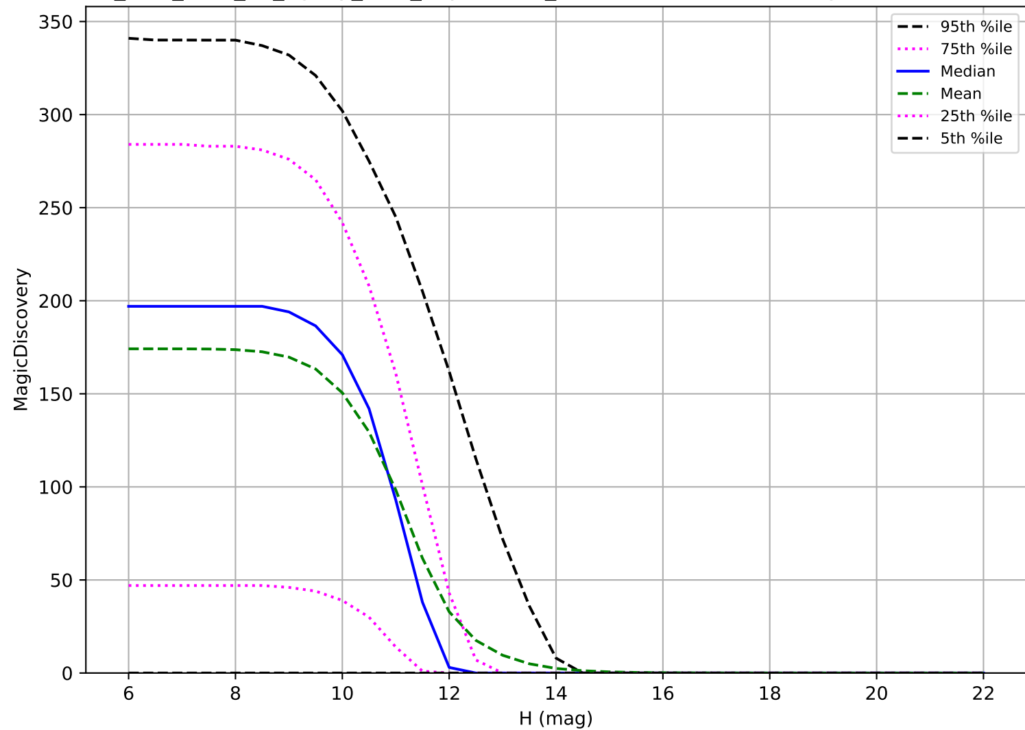
too_elab_r256_d2_ugrizy_v3.4_10yrs: OCC_r20 6 detections in 60 nights detection loss
