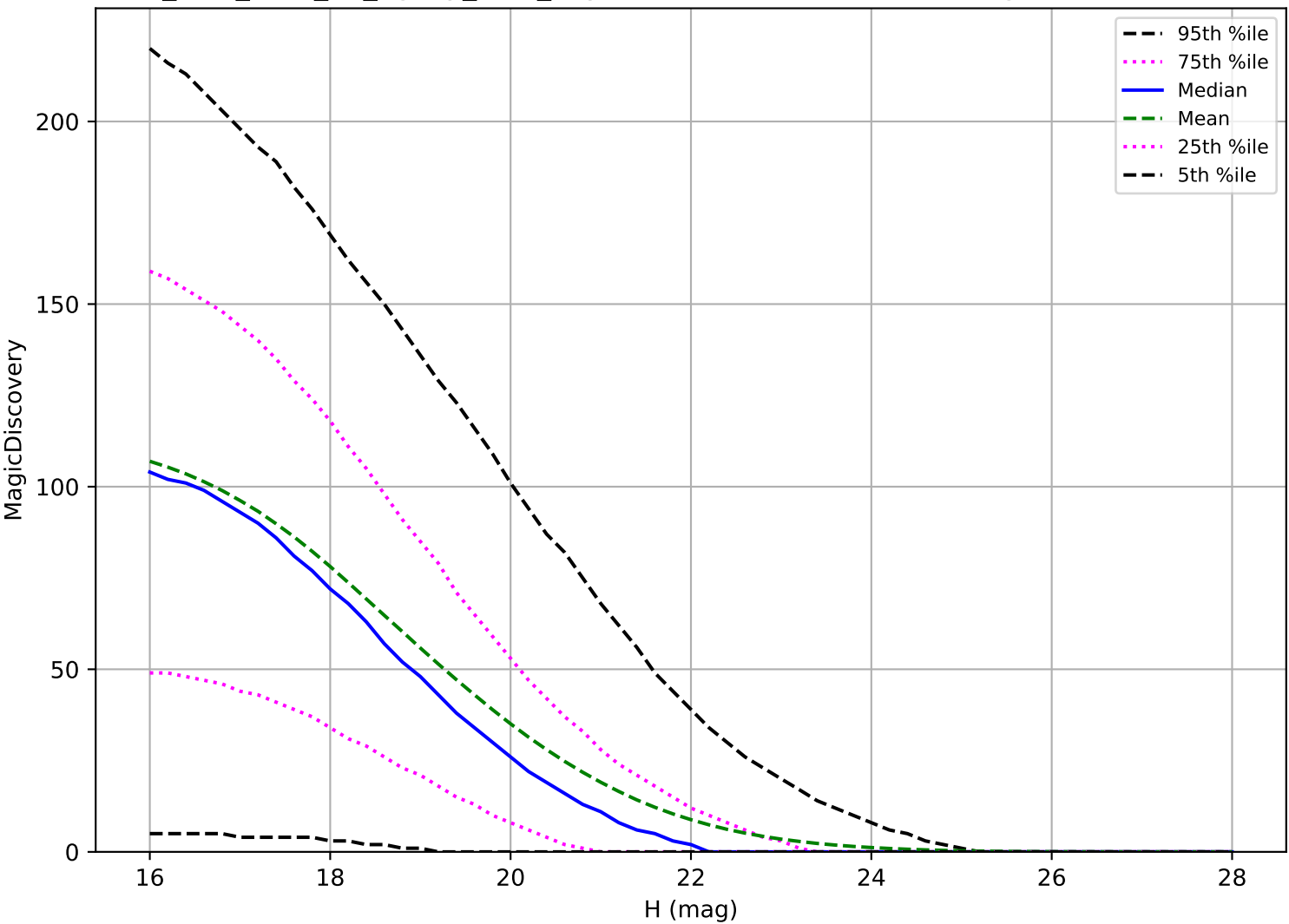
too_elab_r256_d2_ugrizy_v3.4_10yrs: NEO 6 detections in 60 nights detection loss
