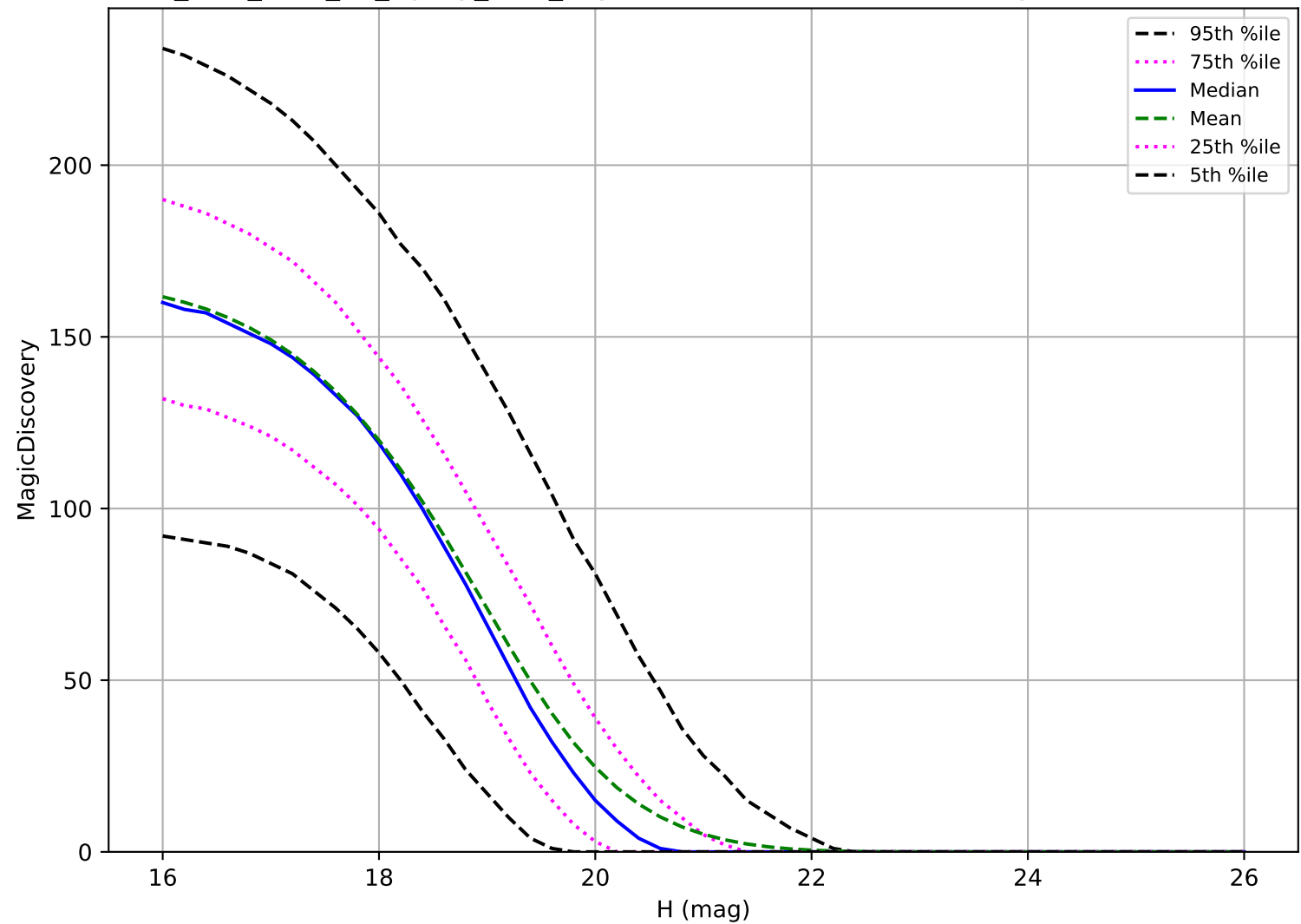
too_elab_r256_d2_ugrizy_v3.4_10yrs: MBA 6 detections in 60 nights detection loss
