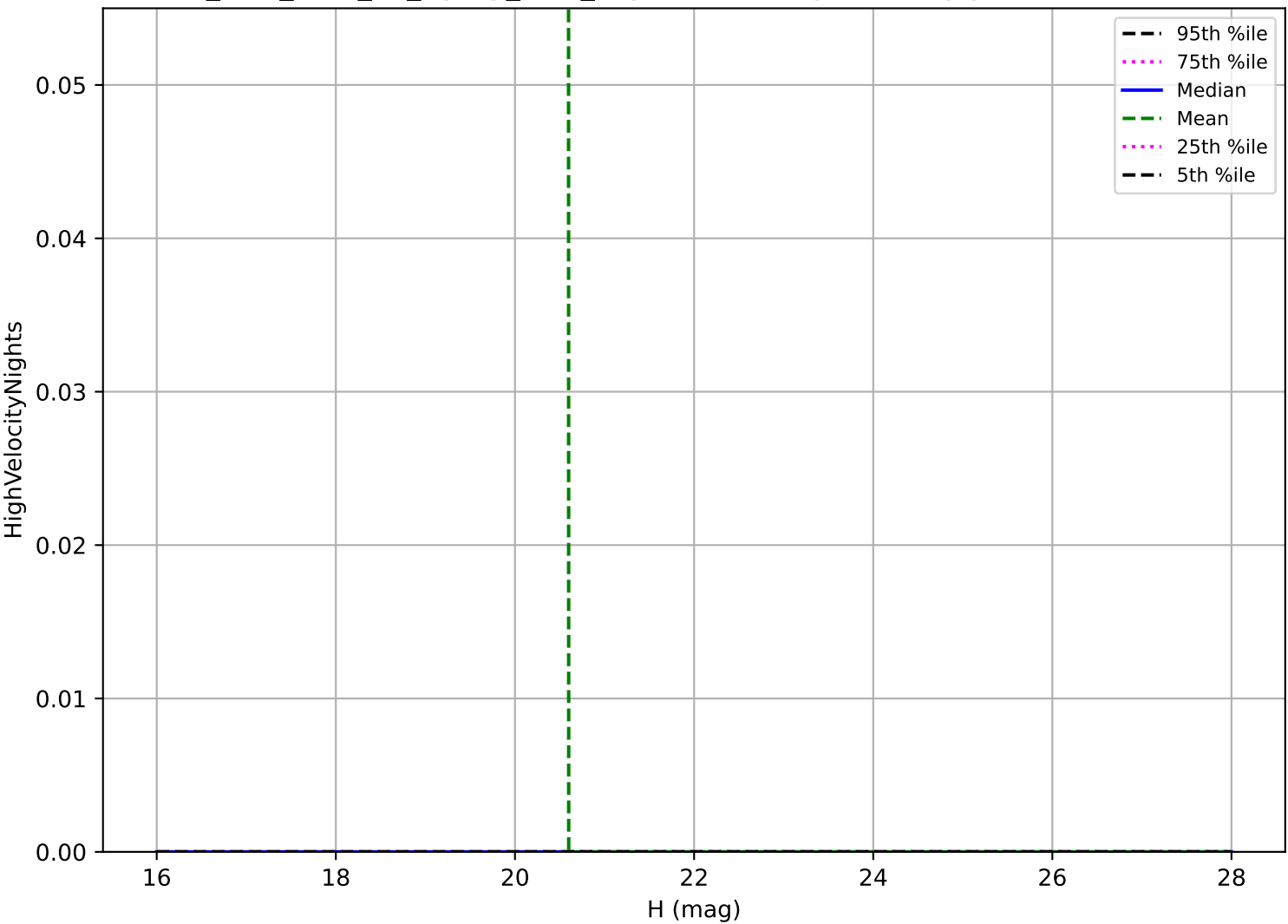
too_elab_r256_d2_ugrizy_v3.4_10yrs: Vatira High velocity pair detection loss
