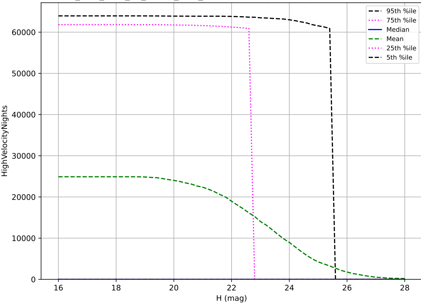
too_elab_r256_d2_ugrizy_v3.4_10yrs: PHA High velocity pair detection loss
