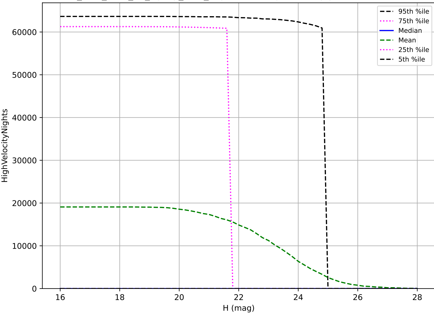
too_elab_r256_d2_ugrizy_v3.4_10yrs: NEO High velocity pair detection loss
