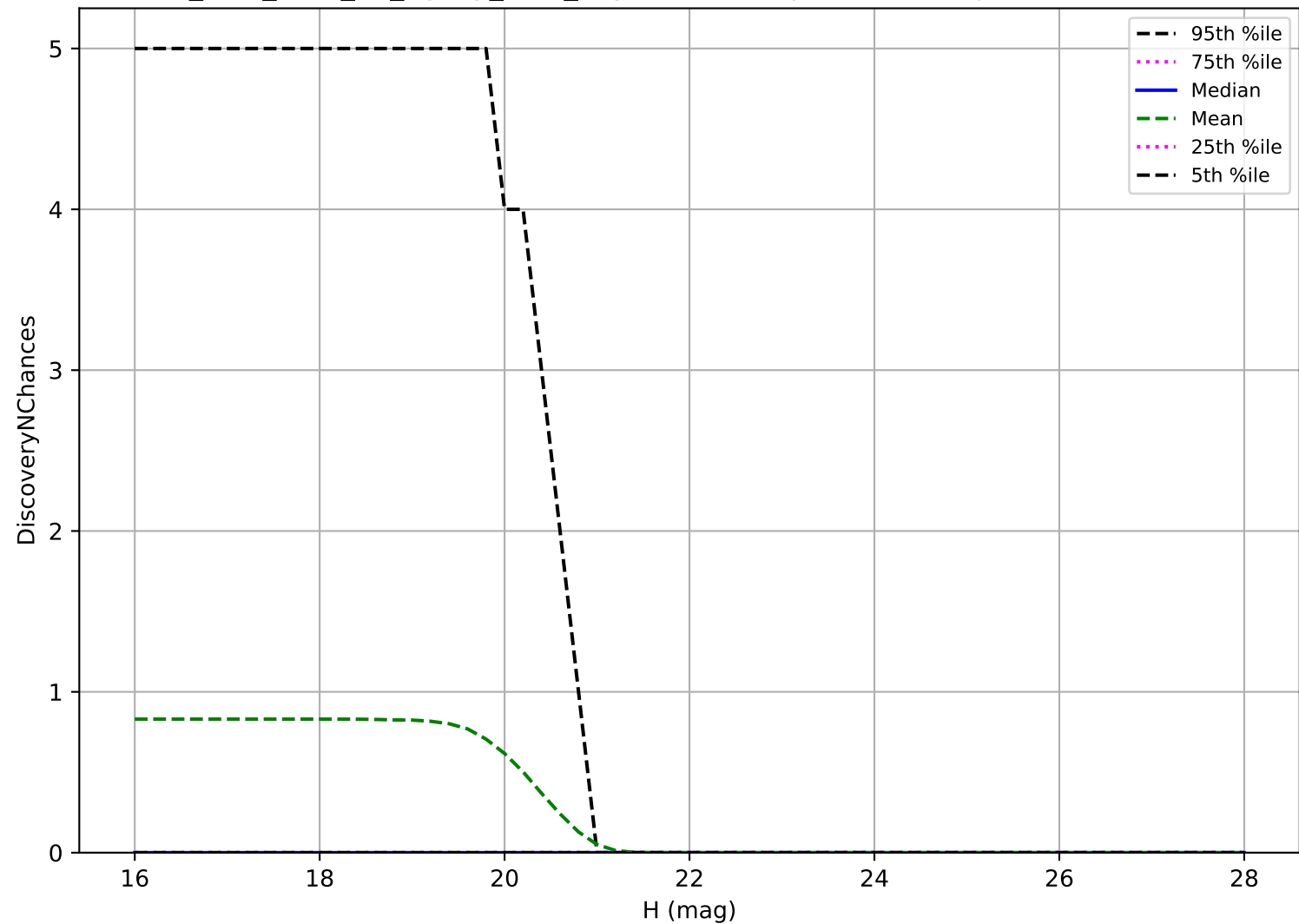
too_elab_r256_d2_ugrizy_v3.4_10yrs: Vatira 3 pairs in 15 nights detection loss
